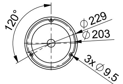
Floor Flange Detail
