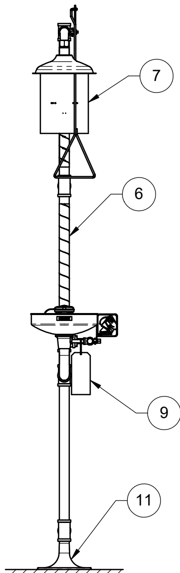
DETAIL A SCALE 1 : 3
