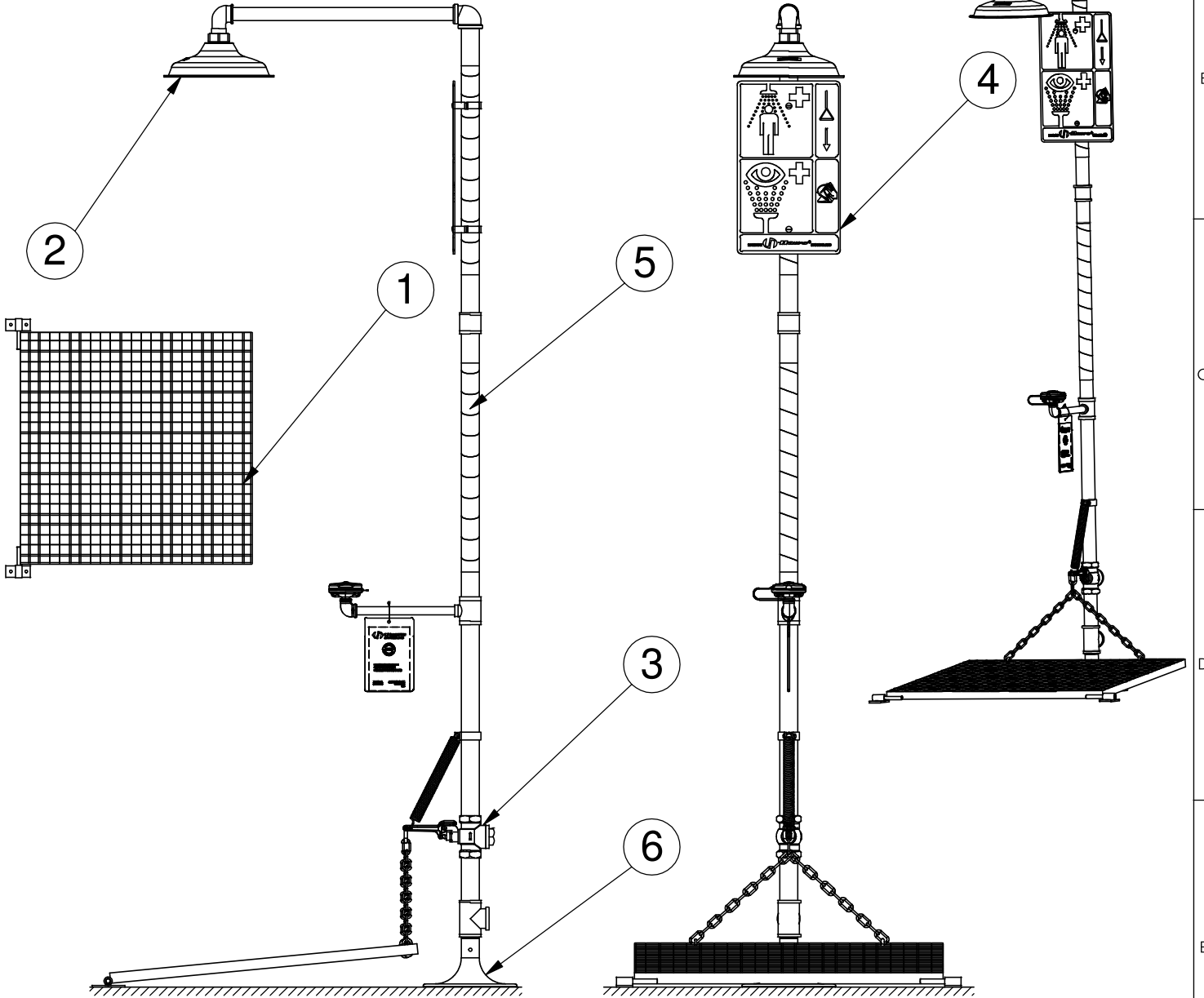
SP65 EYE WASH ASSEMBLY
